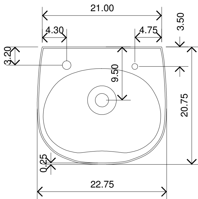
Bottom (Bowl outline shown level with bottom of outer edge)
